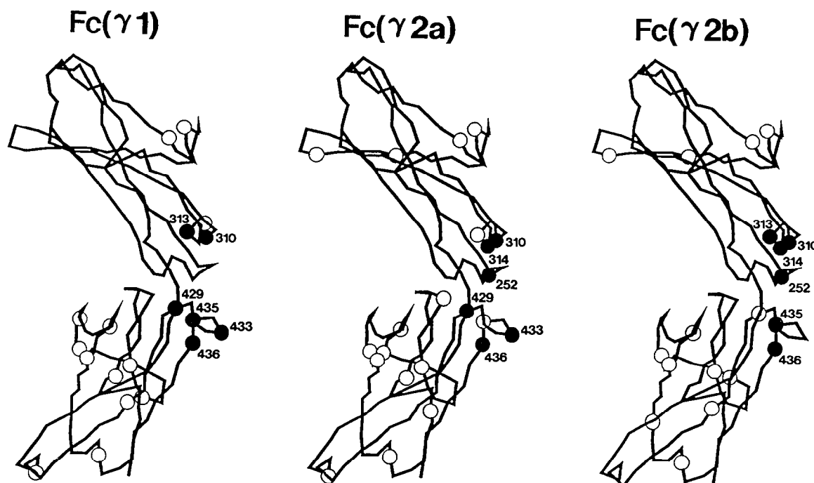
Fig. 3. Mapping of the FB binding site on Fc( \gamma 1), Fc( \gamma 2a), and Fc( \gamma 2b) by use of chemical shift changes of the carbonyl ^{13}\text{C} resonances of His, Met, Trp, and Tyr induced by addition of FB as spectroscopic probes. Chemical shift changes were observed at pH 8.8, 7.0, and 6.5 for Fc( \gamma 1), Fc( \gamma 2a), and Fc( \gamma 2b), respectively. Positions of the residues showing chemical shift changes larger (closed circles) and less (open circles) than 0.1 ppm are presented on the crystal structure of the human IgG Fc fragment deposited in Brookhaven Protein Data Bank [4]. Although four Tyr resonances have not been assigned in the case of Fc( \gamma 2a) as described in the text, both of Tyr resonances originating from the Tyr-Ser dipeptide (Tyr-407 and Tyr-423) were shifted less than 0.1 ppm in the presence of FB and therefore are included as such in the figure.
