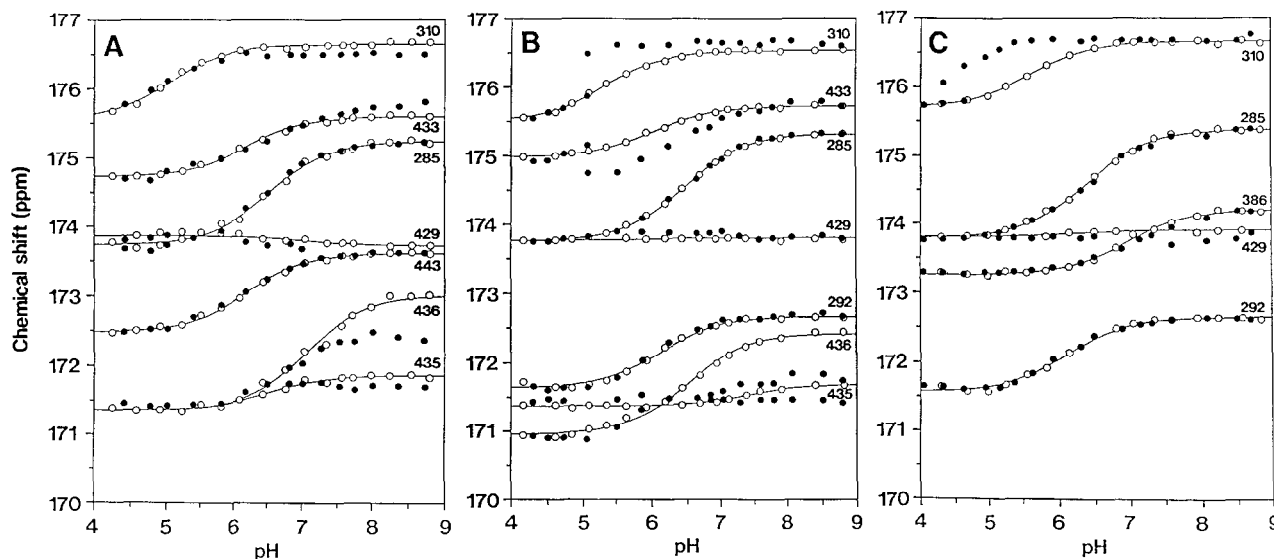
Fig. 1. The pH dependence of the chemical shift of the histidyl carbonyl ^{13}\text{C} resonances of (A) Fc( \gamma 1), (B) Fc( \gamma 2a), and (C) Fc( \gamma 2b) in the absence (open circles) and presence (closed circles) of FB. The molar ratio of Fc/FB was 1.2.
